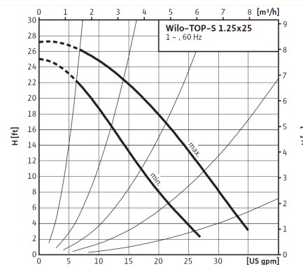
Sample Pump Curve showing Recommended Wilo TOP-S-1.25x25 Circulator
