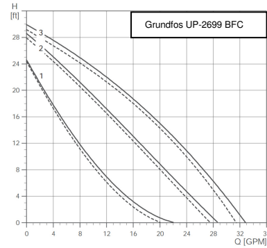
Sample Pump Curve showing Popular Grundfos UP-2699-BFC Circulator
